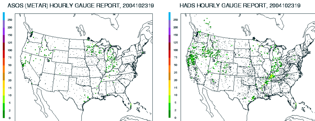
Fig. 2. Hourly ASOS (METAR) and HADS gauge reports valid at 2004102319. Black dots are reports of zero precipitation.
