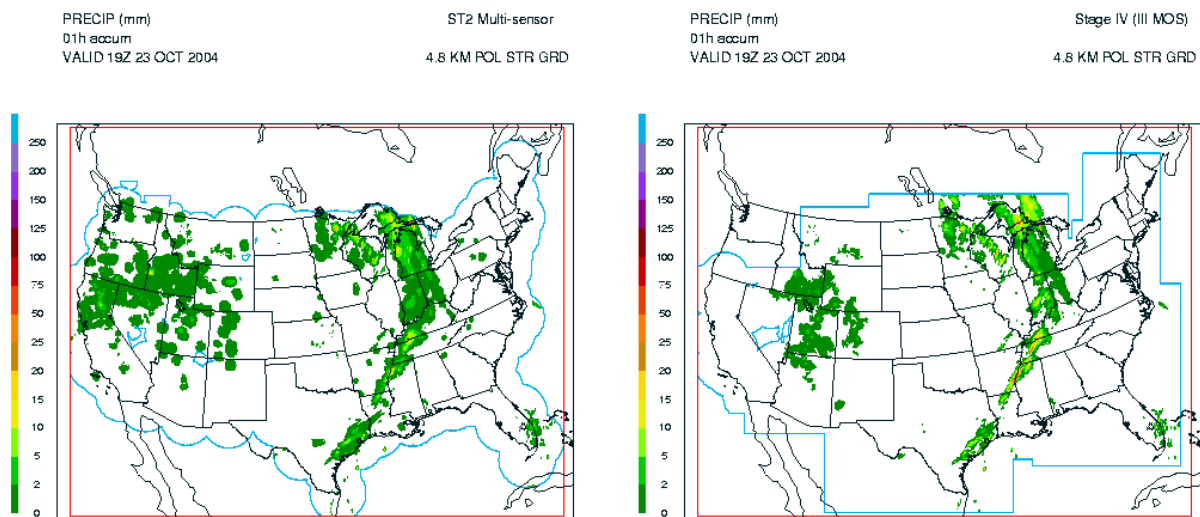
Fig. 1 Snapshot of a one-hour Stage II (left) and Stage IV (right) analysis.
