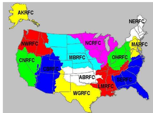
Fig. 3. RFC domains. Image from http://www.srh.noaa.gov/lub/wx/nows_HSAs.htm
