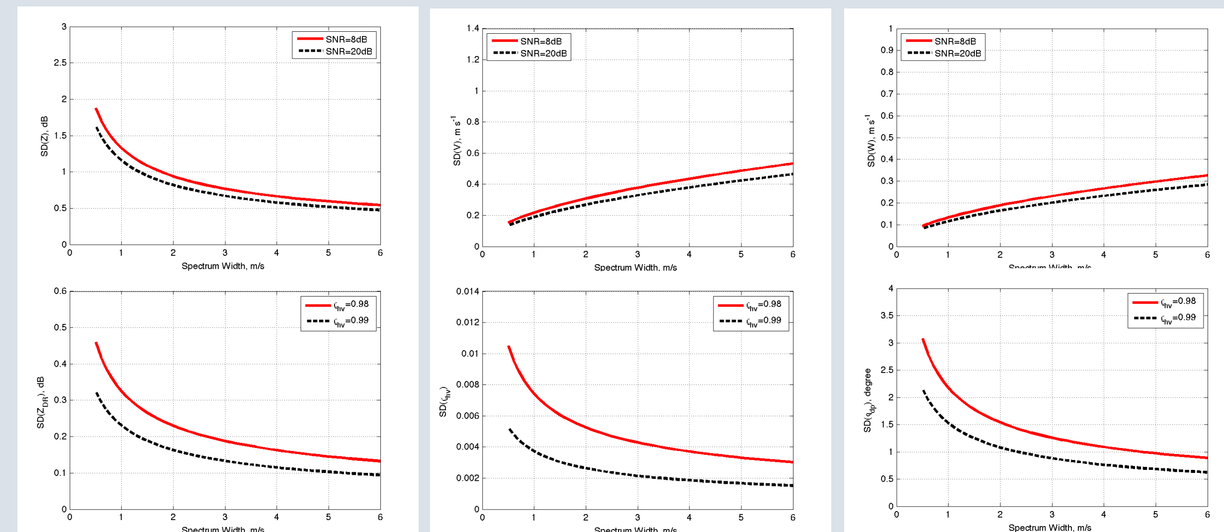
Figure 1. Example of C-band (5 cm) radar theoretical sampling-induced errors (SD values) for six moments: Z, V, W, Z_{DR} , \Phi_{dp} , and \rho_{hv} . The dwell time is 100 ms (e.g., PRF=600Hz, sample number=60). Low SNRs (or \rho_{hv} ) would enlarge the errors.
