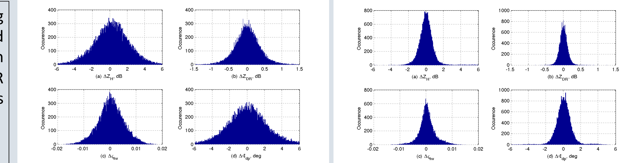
Figure 6. The histogram of the moment differences between two consecutive rays: (a) \Delta Z_H , (b) \Delta Z_{DR} , (c) \Delta \rho_{hv} , and (d) \Delta \Phi_{dp} . The data were collected with setting one and limited by 0.1 < W < 2 m/s. The histograms show a large variation of sample difference.
