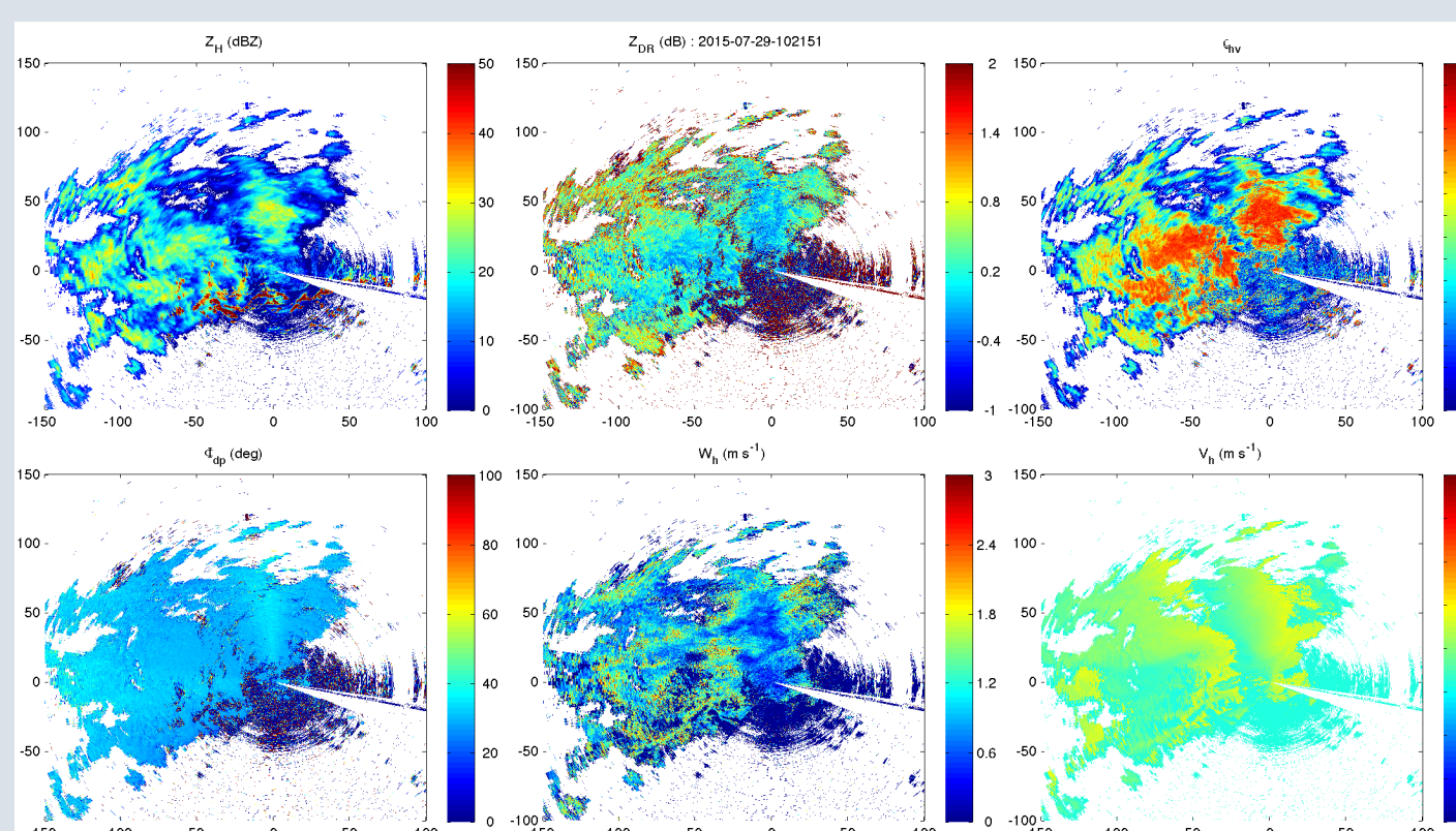
Figure 3. Same as Fig. 2 except for using the setting two (10:21:51UTC, 29 July 2015). The velocity-aliasing is clearly seen but the data quality of all the moments looks better.
