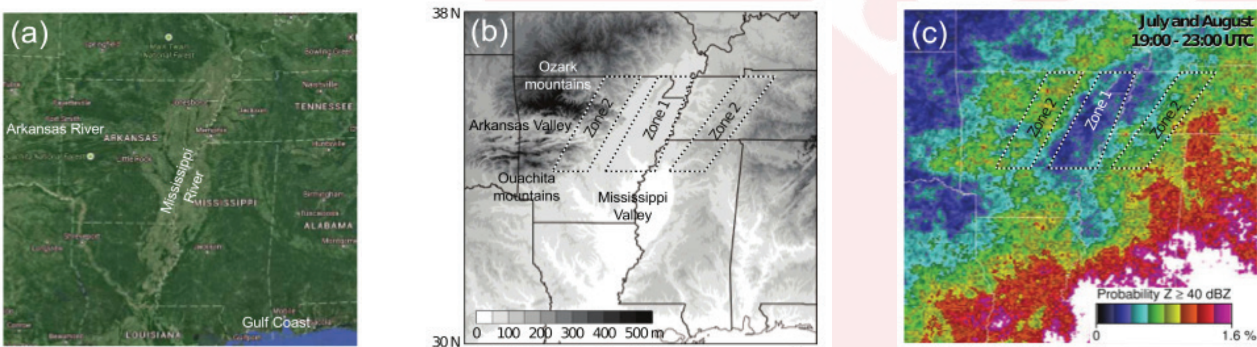
Fig. A.1. : Satellite image of Mississippi Valley (courtesy of Google Maps) (a), terrain height (b), and probability of occurrence of reflectivity over 40 dBZ in mid-afternoon (19 – 23 UTC) in July and August derived from the US radar composites.
