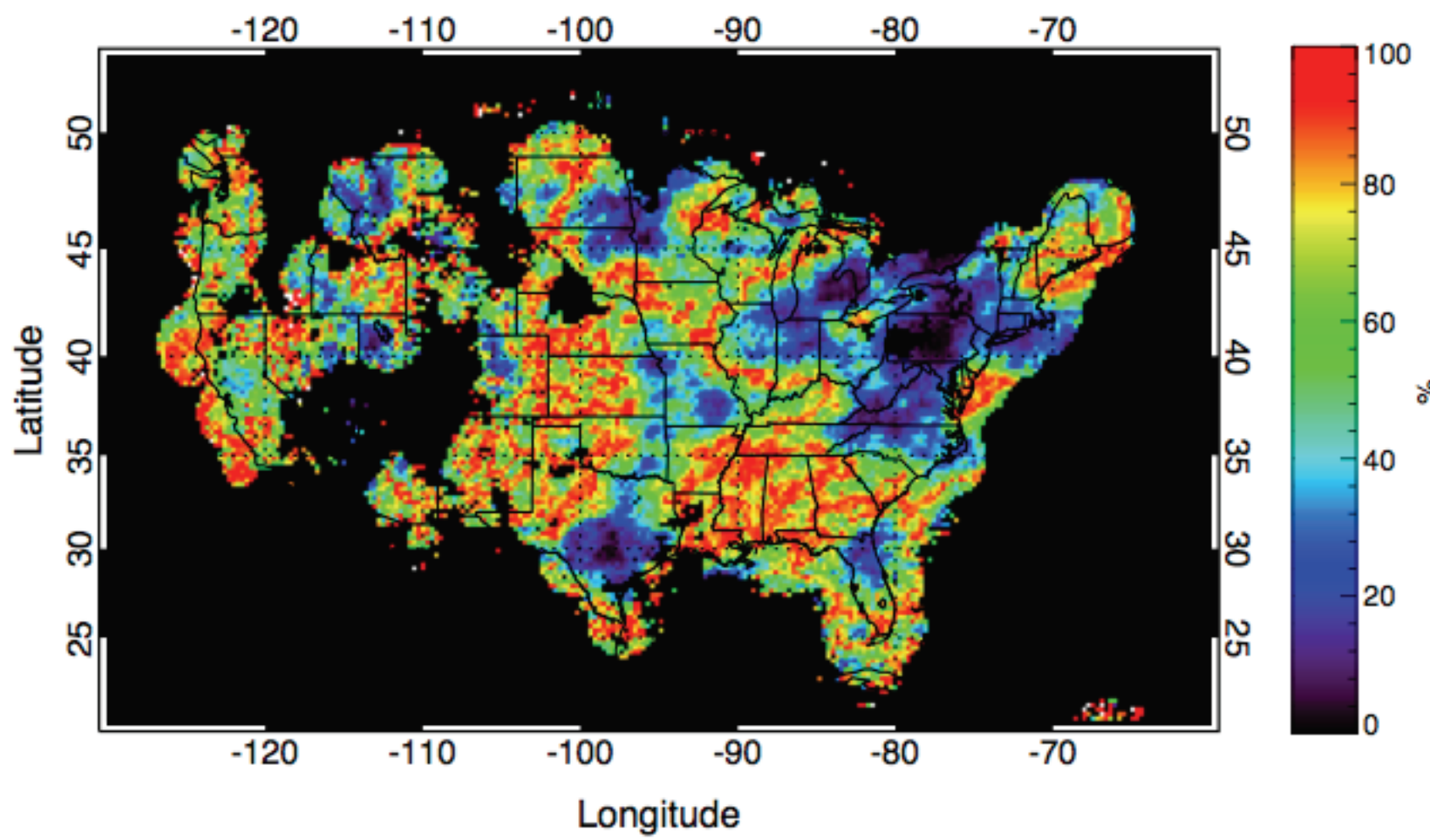
Probability of having common results between weekday and weekend
