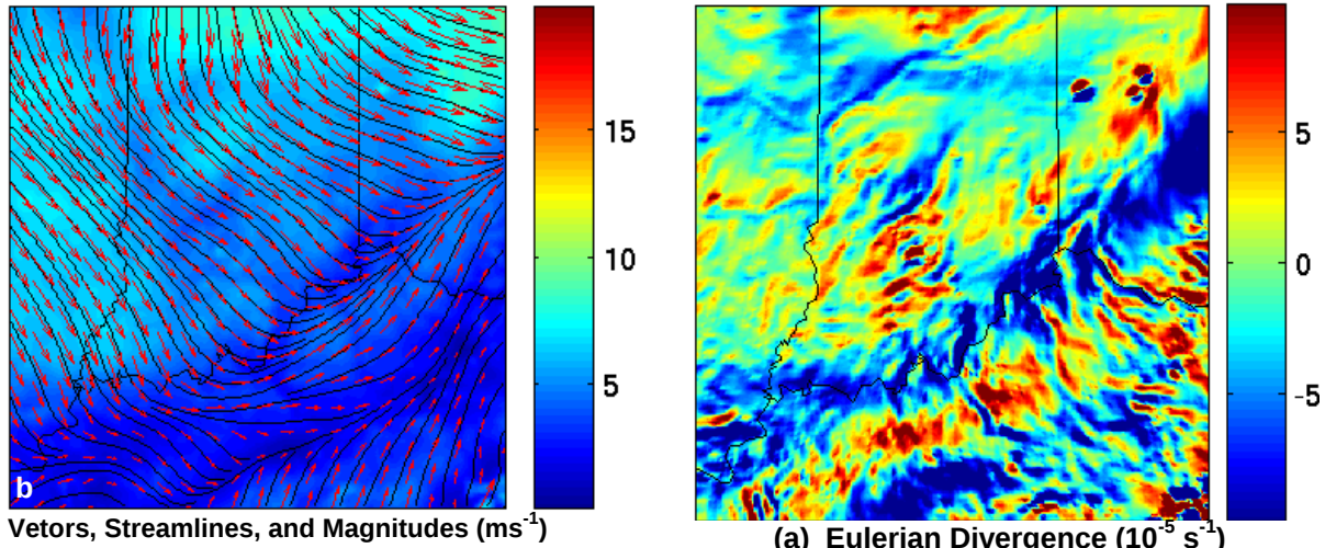
Figure 6a and b. Surface wind observations (a) and the STMAS wind analysis (b) valid 23:00 UTC on March 7 th 2005.
