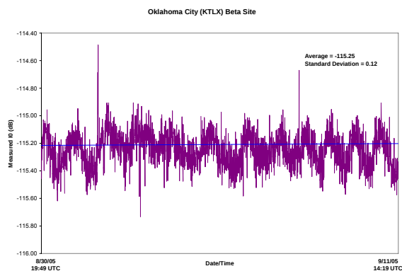
Figure 10: KTLX I_0
