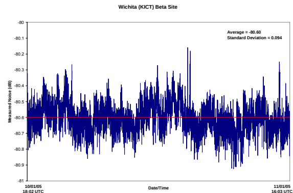
Figure 6: KICT Noise Measurements
