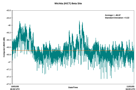
Figure 13: KICT Calibration
