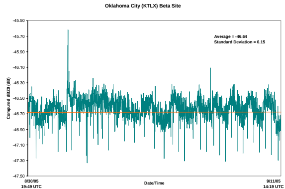
Figure 11: KTLX Calibration
