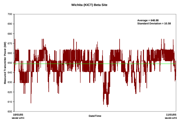
Figure 8: KICT Transmitter Power
