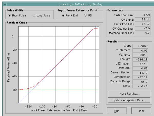
Figure 9: Receiver Transfer Curve
