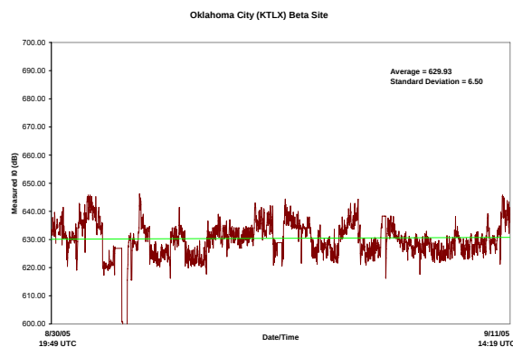
Figure 7: KTLX Transmitter Power
