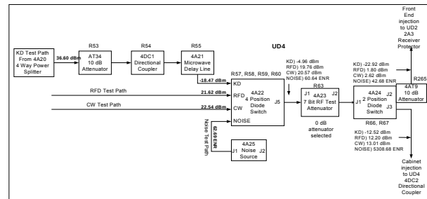
Figure 2: ORDA Test Path
