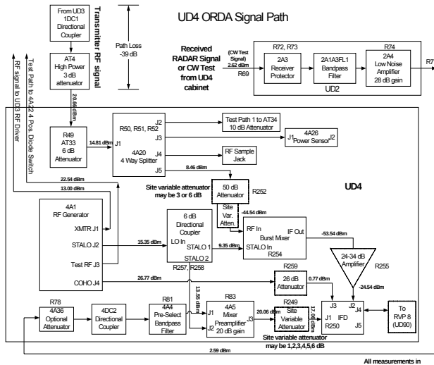
Figure 1: ORDA Receiver Signal Path
