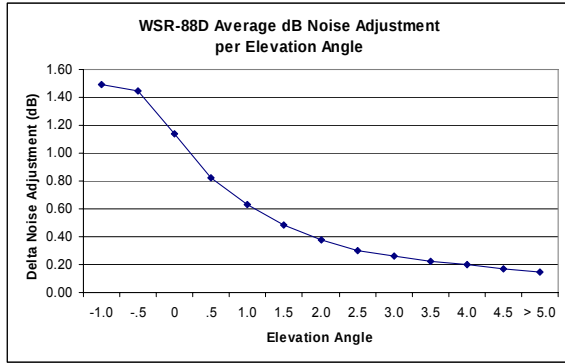
Figure 4: Noise Adjustment per Elevation Angle
