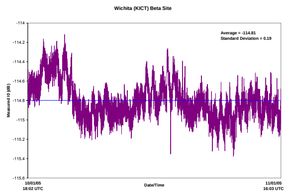
Figure 12: KICT I_0
