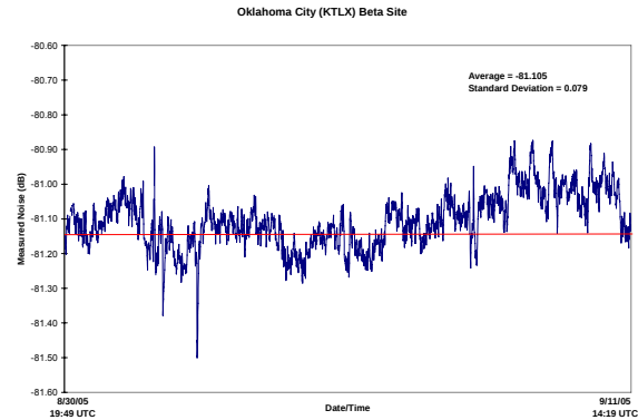
Figure 5: KTLX Noise Measurements
