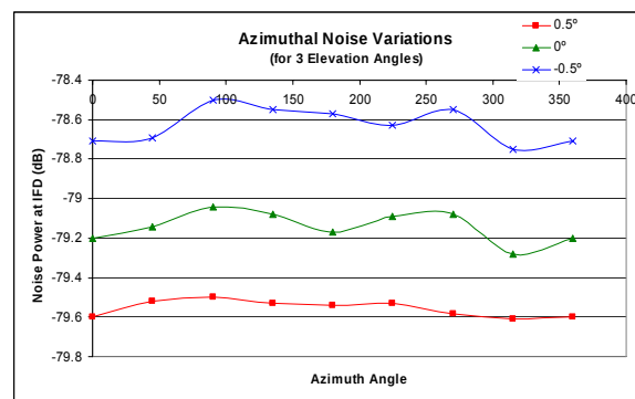
Figure 3: Azimuth and Elevation Noise Changes
